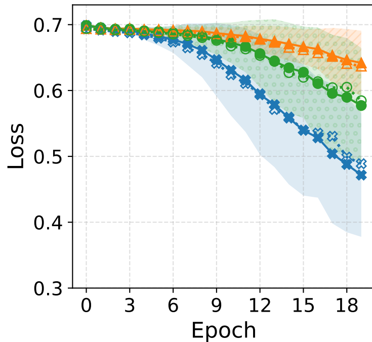
Model: QCNN with Classical NN
